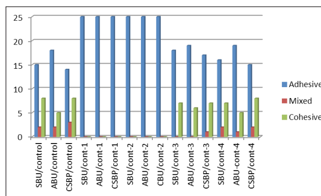
Figure 3: Failure modes
